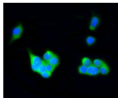
Fig. 2. ICC staining Rab4A in PC-12 cells (green). The nuclear counter stain is DAPI (blue). Cells were fixed in paraformaldehyde, permeabilised with 0.25% Triton X-100/PBS.
