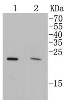
Fig. 1. Western blot analysis of Rab4A on different cell lysates using anti-Rab4A antibody at 1/500 dilution. Positive control :Lane 1: MCF-7; Lane 2: 293T
